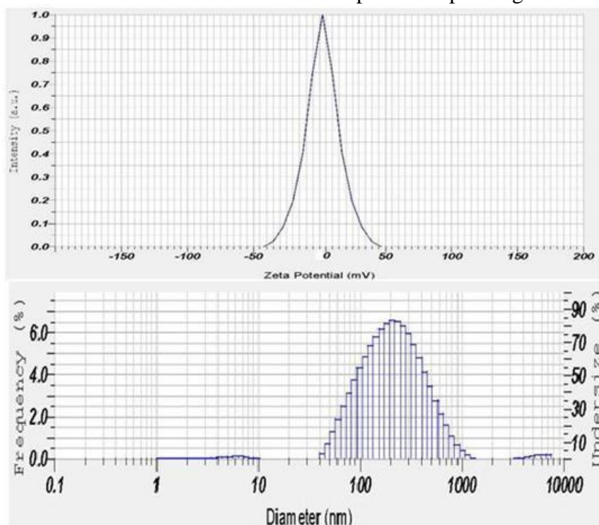
Fig. 8: Zeta Potential of the Microemulsion Formulation (F1)
