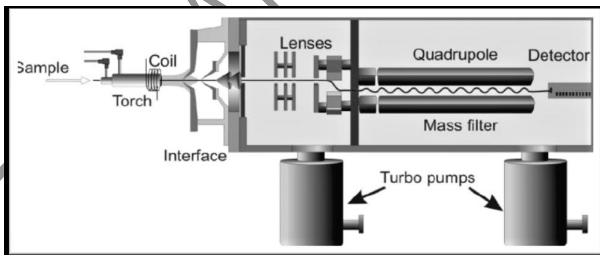
Fig. 1: Single Quadrupole ICP-MS
